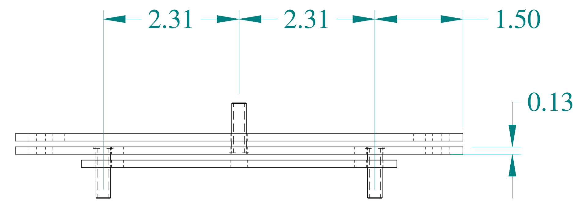
TOP VIEW
