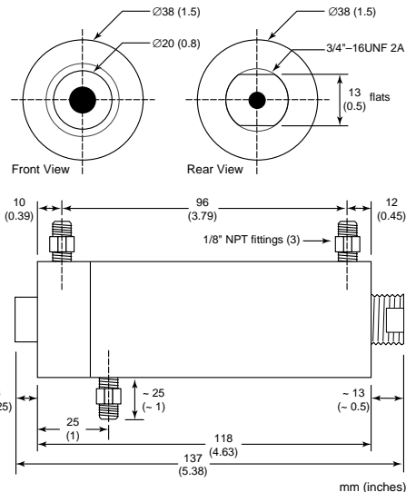
Figure 8: Air/Water-cooled Housing
